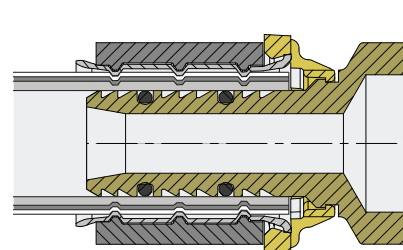
PROFILE U
